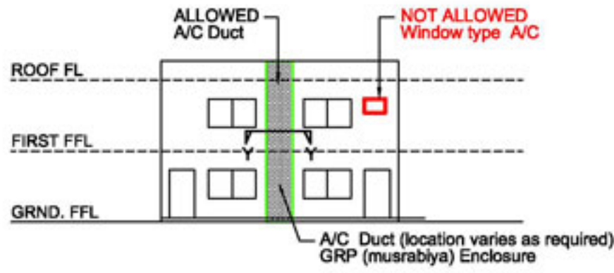
MAIN / FRONT ELEVATION (Villas, Flats & High Rise Buildings)
